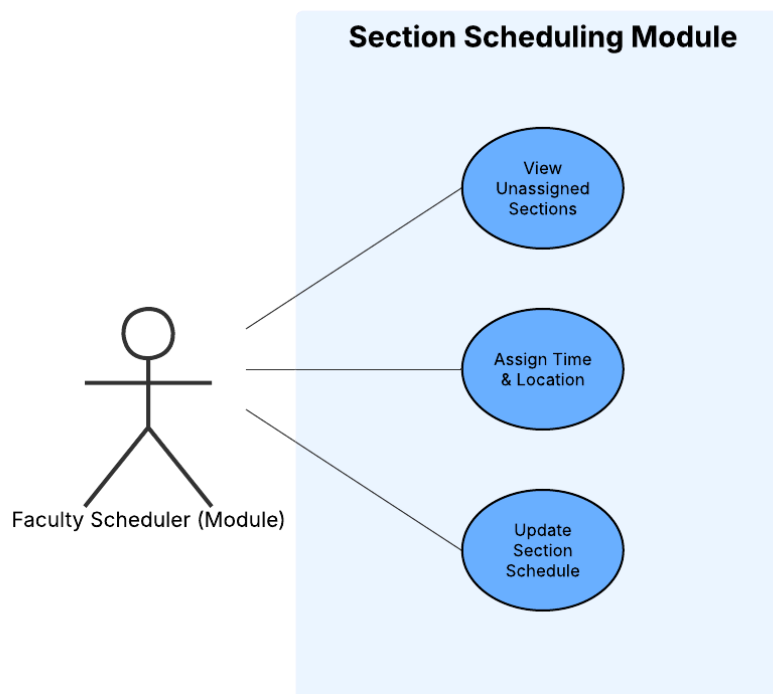
Figure 4.12: Use Case Diagram for Section Scheduling Module
