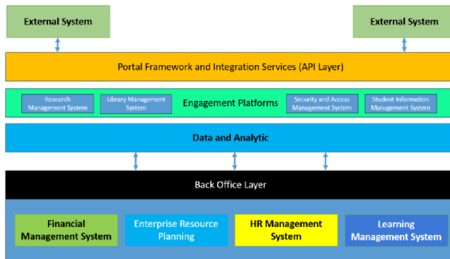
Figure 2.2.2.1: Enterprise Architecture by Hidarto. Hidarto (2023)
