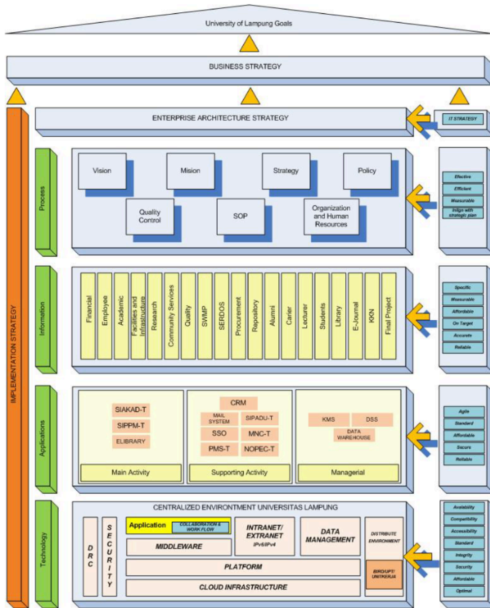
Figure 2.2.1: Enterprise Architecture proposed to Unila. (Nama & Kurniawan, 2023)
