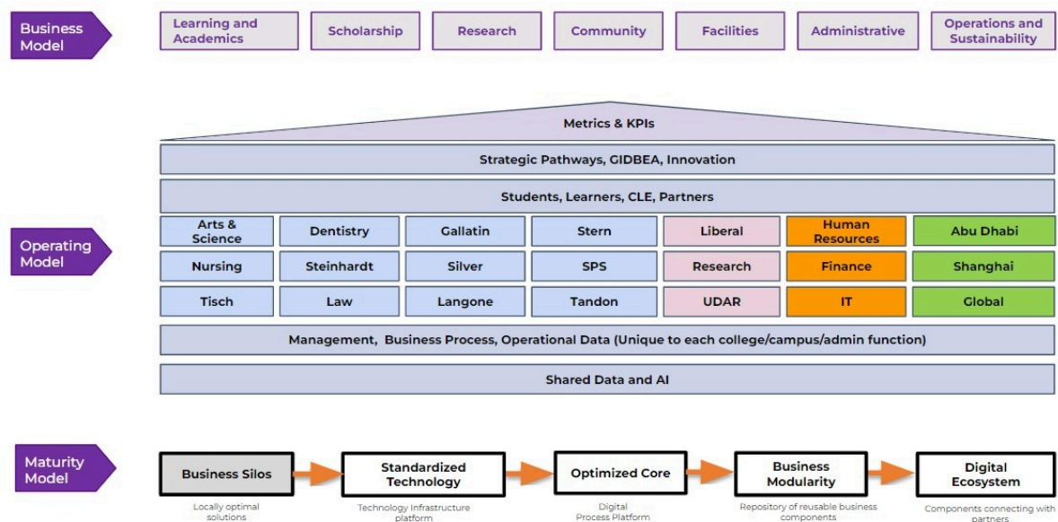
Figure 2.2.3.1: Enterprise Architecture New York University
